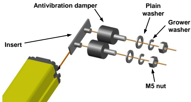
SIDE ASSEMBLY
