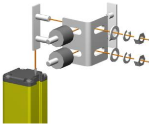
SIDE ASSEMBLY
